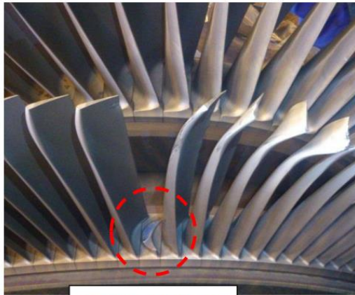
Fatigue failure
